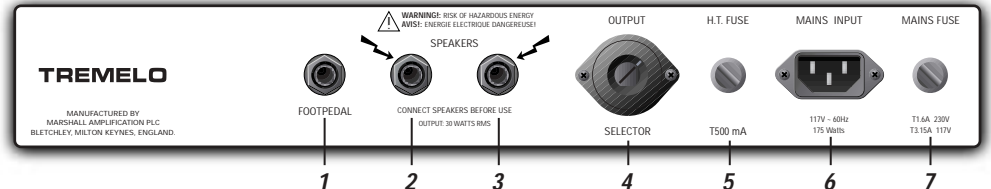
1962 Rear Panel
